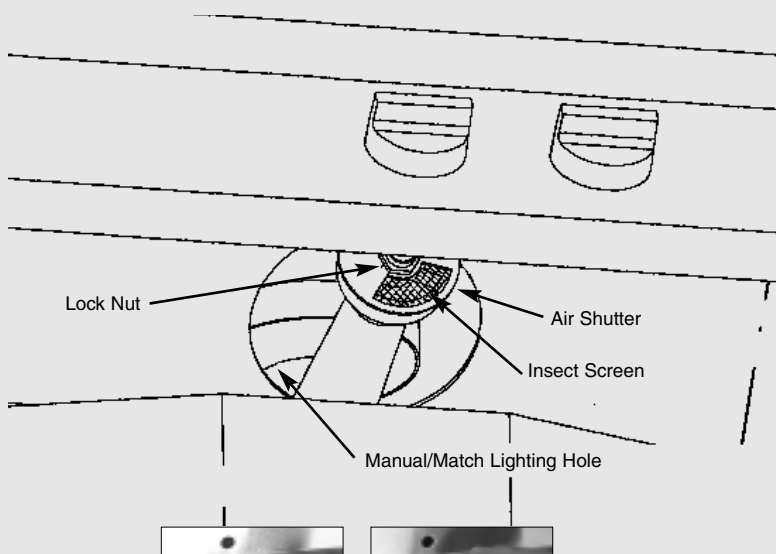
FIGURE 6 CUTAWAY VIEW
